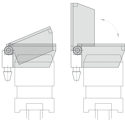
Structure of the protective flaps on the front panel
